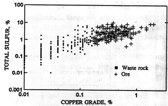
Figure 2. Sulfur versus copper grade
