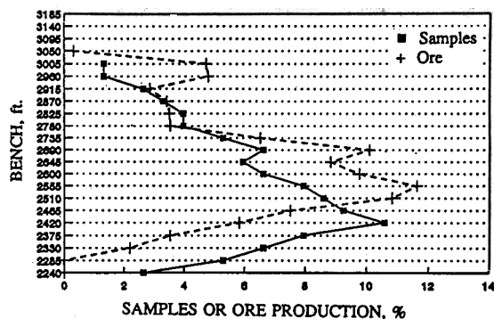
Figure 9. Percent samples and production by bench.
